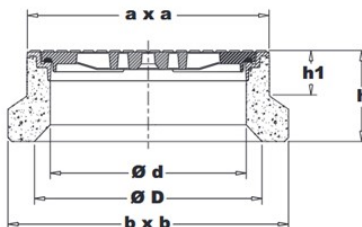
type N 352 NB-RR Centerfix 170 - 240 mm
