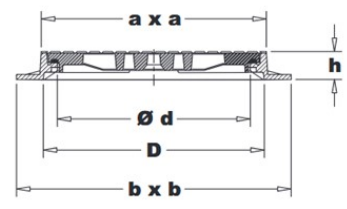
type N 352 NG-RR Centerfix 75 mm
