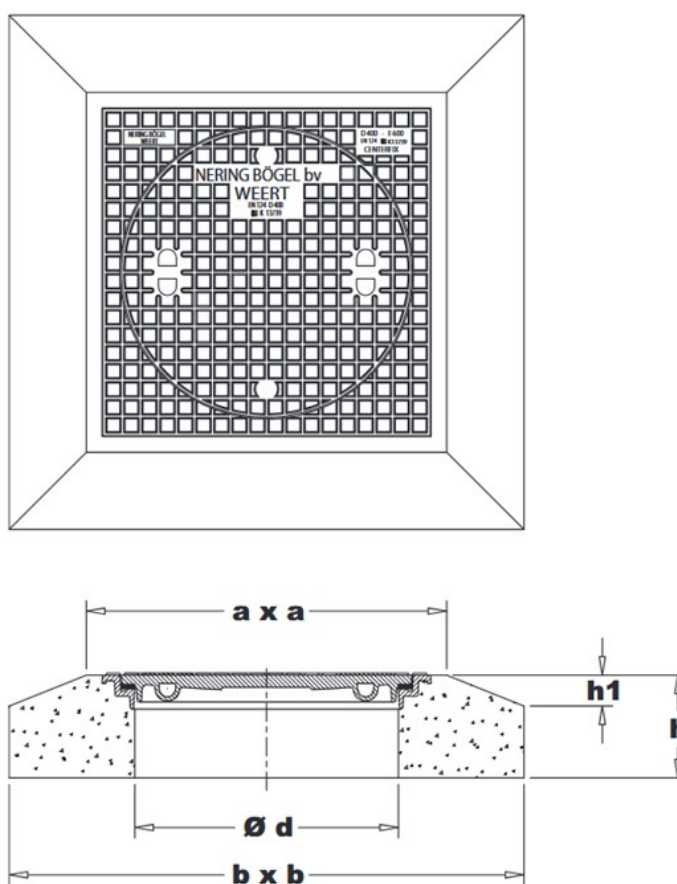
type N 352 NB-R-BERM Centerfix
