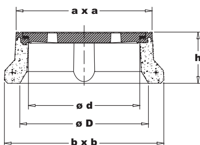
type N 362 NB-RR Centernorm
