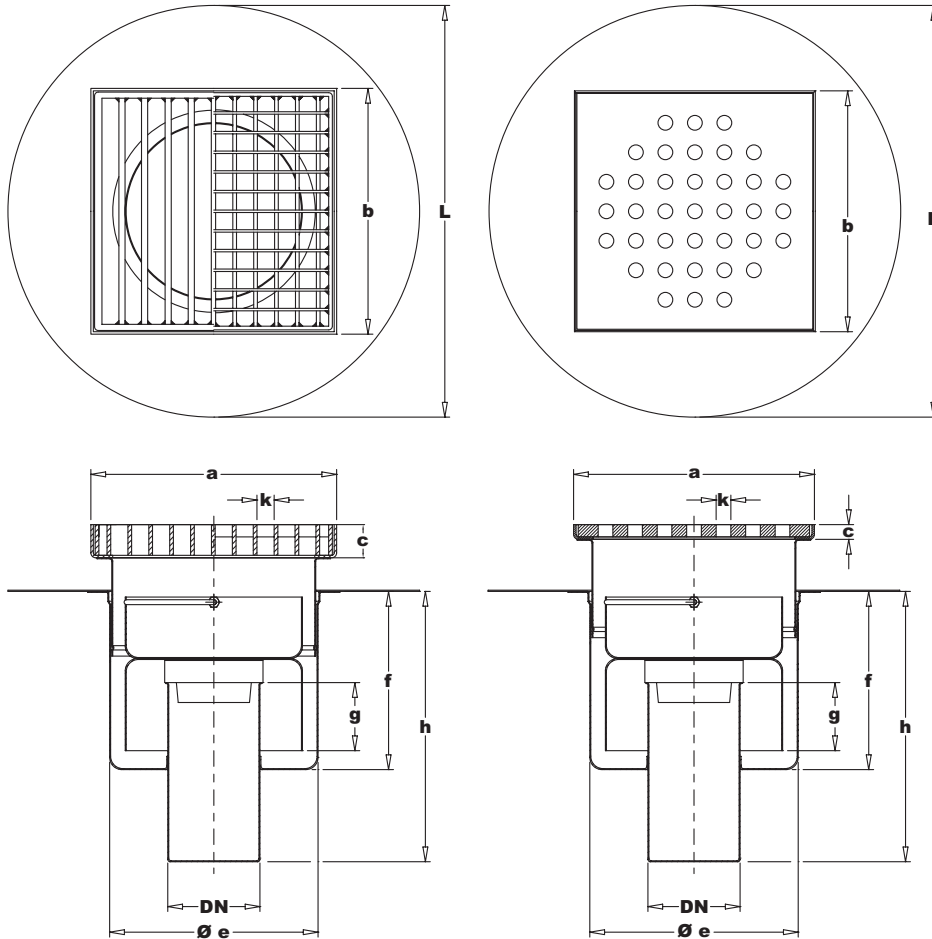
type 1121 RFZM - 1131 RFZM type 1121 RFZS
