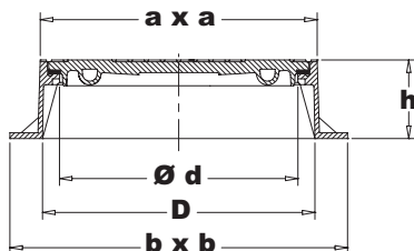
type N 352 NG-R Centerfix 100 - 175 mm
